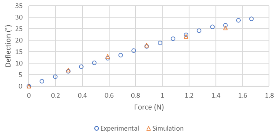
15 Turn Hexagon Spring 3x Semi-Scaled PLA Simulation Validation
