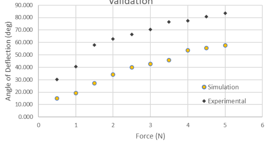
Variable Pitch 3x Semi-Scaled PLA Simulation Validation
