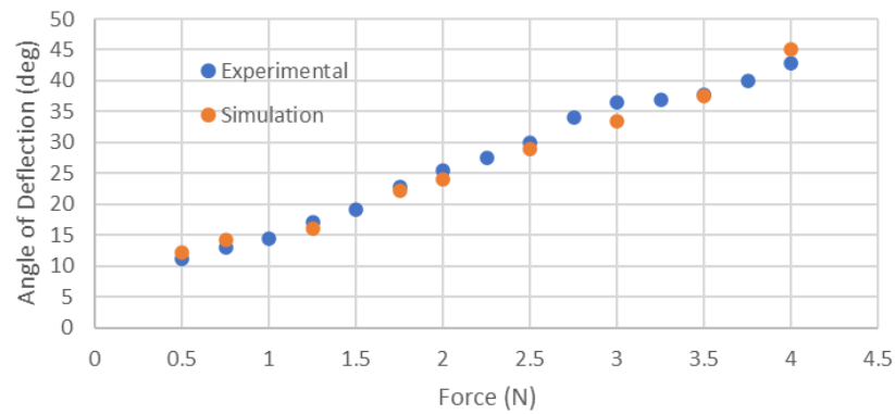
Circle with Ellipse 3x Semi-Scaled Simulation Validation
