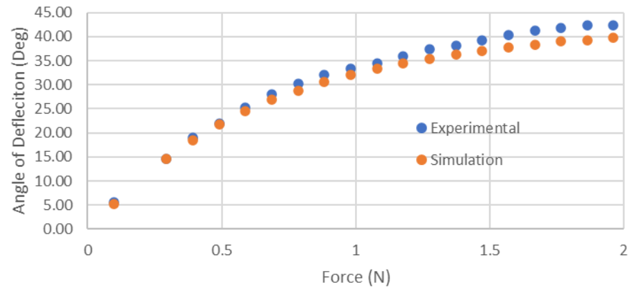
Reverse Hourglass 3x Semi-Scaled PLA Simulation Validation
