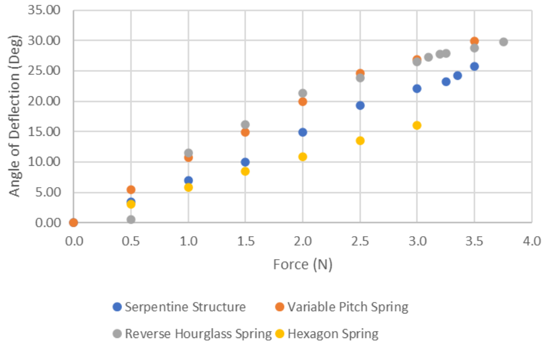
True Size Aluminum 6061-T6 Angle of Deflection Comparison
