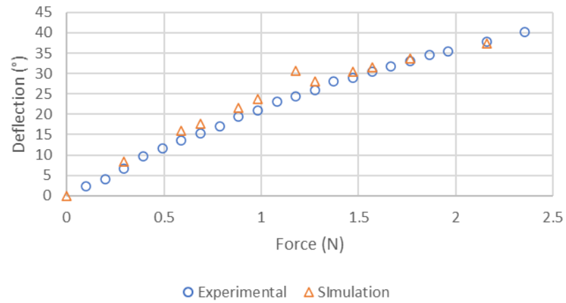
18 Turn Hexagon Spring 3x Semi-Scaled PLA Simulation Validation
