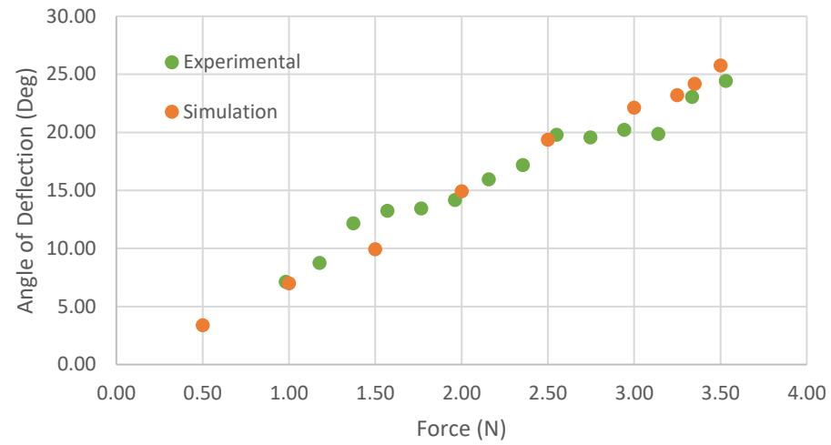
Serpentine 3x Scaled PLA Simulation Validation
