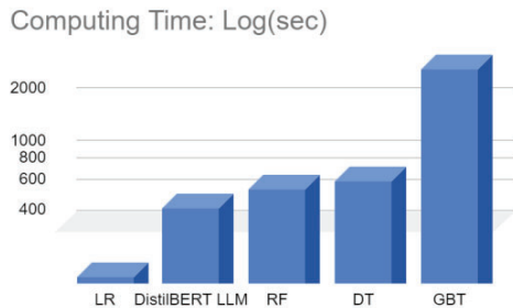
Fig. 1. Computing Time of the Models
