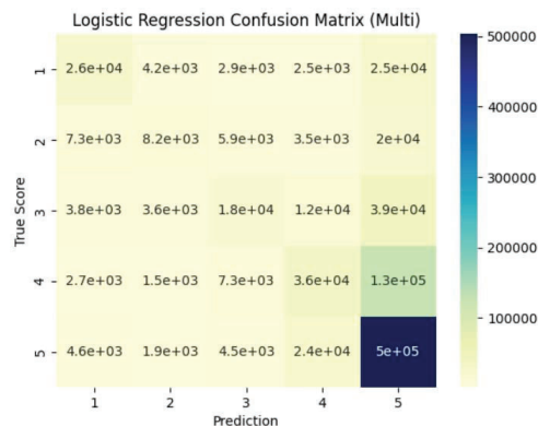
Fig 2. Confusion Matrix of Multiclass LR
