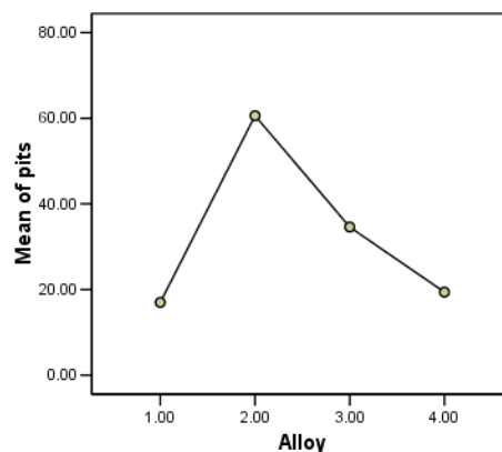
Figure 18 – Means Plot
