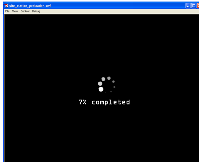
Figure 37 – Preloader
