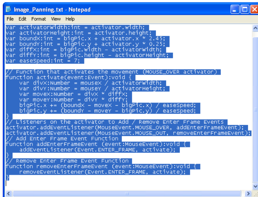
Figure 28 – Image_Panning.txt File
