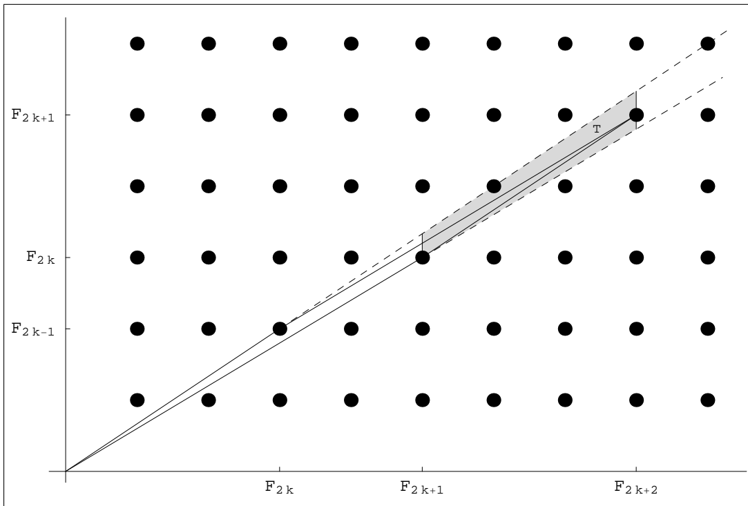
FIGURE 1. Ratios of consecutive Fibonacci numbers
