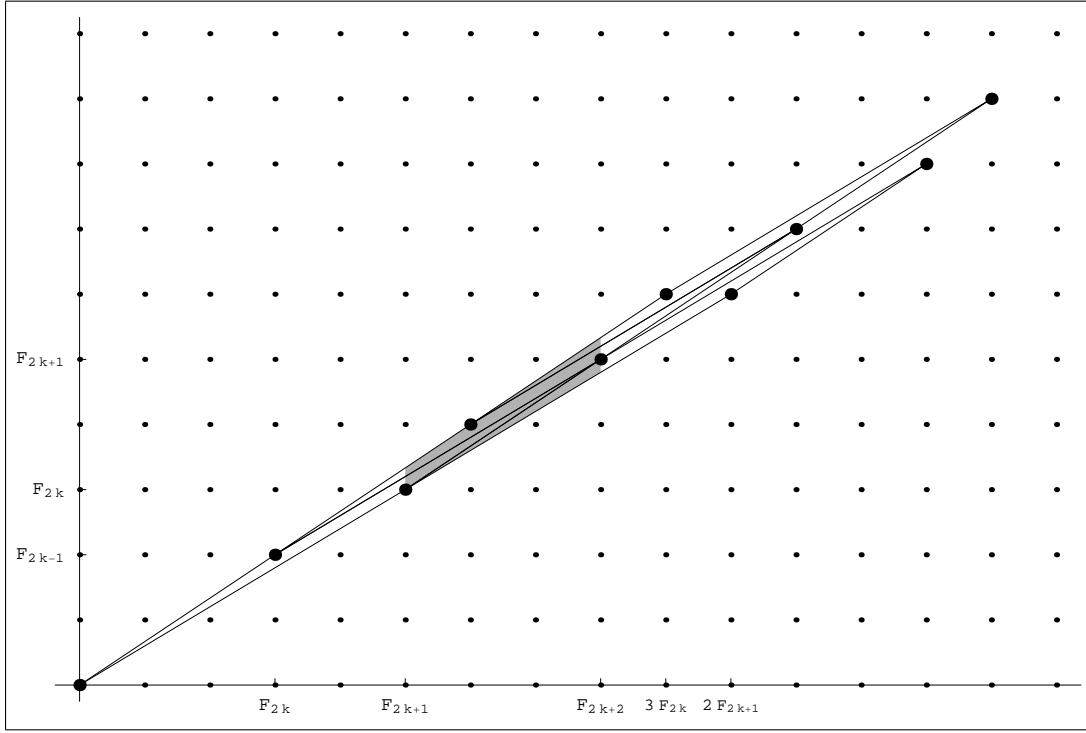
FIGURE 3. Four parallelograms cover T
