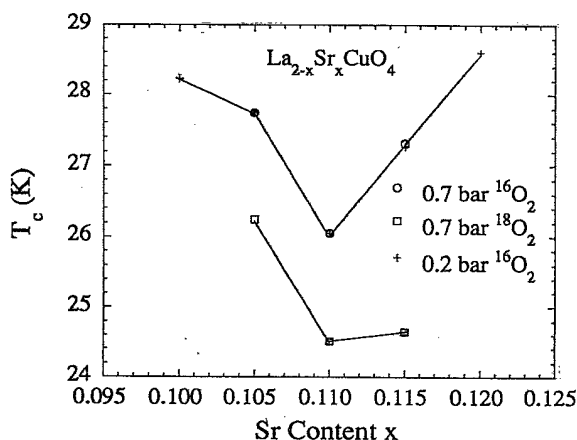
FIG. 2. The superconducting transition temperatures T_c vs x for the ^{16}\text{O} and ^{18}\text{O} samples of \text{La}_{2-x}\text{Sr}_x\text{CuO}_4 . Since the T_c values of the ^{16}\text{O} -containing samples have a local minimum at n \approx x \approx 0.110 , any increase or decrease in the hole concentration upon isotope substitution will raise the T_c of the sample at this composition. Therefore, a lowering in T_c of the ^{18}\text{O} sample at this composition is not due to a lower or higher hole concentration in the ^{18}\text{O} sample.
