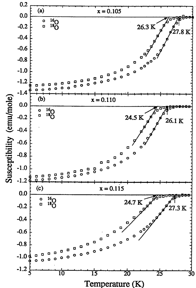
FIG. 1. The FCW susceptibility for the ^{16}\text{O} and ^{18}\text{O} samples of \text{La}_{2-x}\text{Sr}_x\text{CuO}_4 with (a) x = 0.105 ; (b) x = 0.110 ; (c) x = 0.115 . The data shown were divided by a nominal field of 5 Oe and not corrected by demagnetization factors. The real magnetic field for measurements is 5.9 \pm 0.2 Oe.
