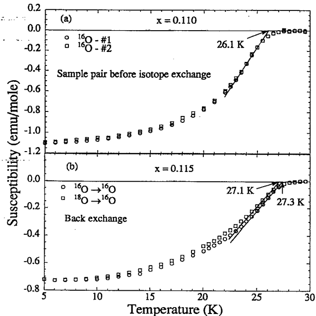
FIG. 3. The FCW susceptibility for the samples of \text{La}_{2-x}\text{Sr}_x\text{CuO}_4 with (a) x=0.110 , before isotope exchange; (b) x=0.115 , after back exchange. The data shown were divided by a nominal field of 5 Oe and not corrected by demagnetization factors. The real magnetic field for measurements is 5.9±0.2 Oe in (a), and 4.1±0.2 Oe in (b).
