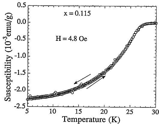
FIG. 4. The temperature dependence of ZFC and FC susceptibility for the x=0.115 sample. The difference of the ZFC and FC signals is small, suggesting negligible flux trapping.
