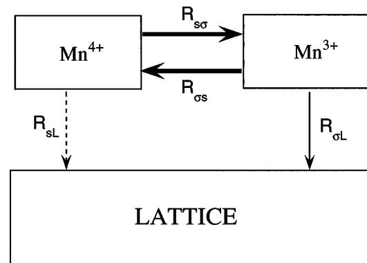
FIG. 4. A Block diagram showing the energy flow paths for the \text{Mn}^{4+} and \text{Mn}^{3+} spin subsystems and the lattice. The relaxation rate R_{ab} represents relaxation from subsystem a to subsystem b . The thickness of the arrows is a measure of the magnitude of the particular relaxation rate R_{ab} .
