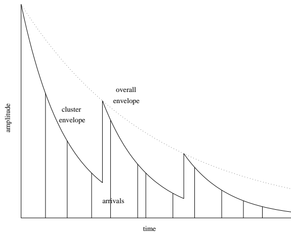
Figure 1. An illustration of exponential decay of mean cluster power and ray power within clusters.
